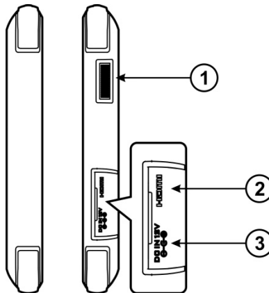
Figure 2-3 MaxiSys Tablet Right Side
